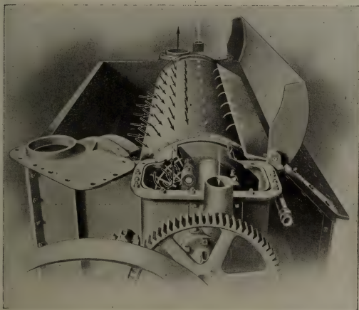
Pneumatic Action of the Save-All
